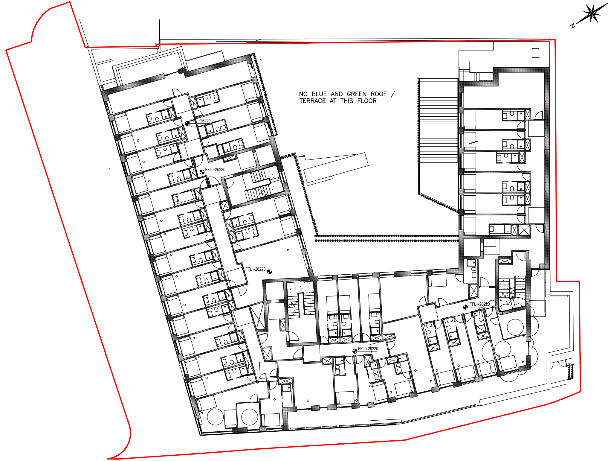
4 FOURTH FLOOR PLAN SCALE 1:250
