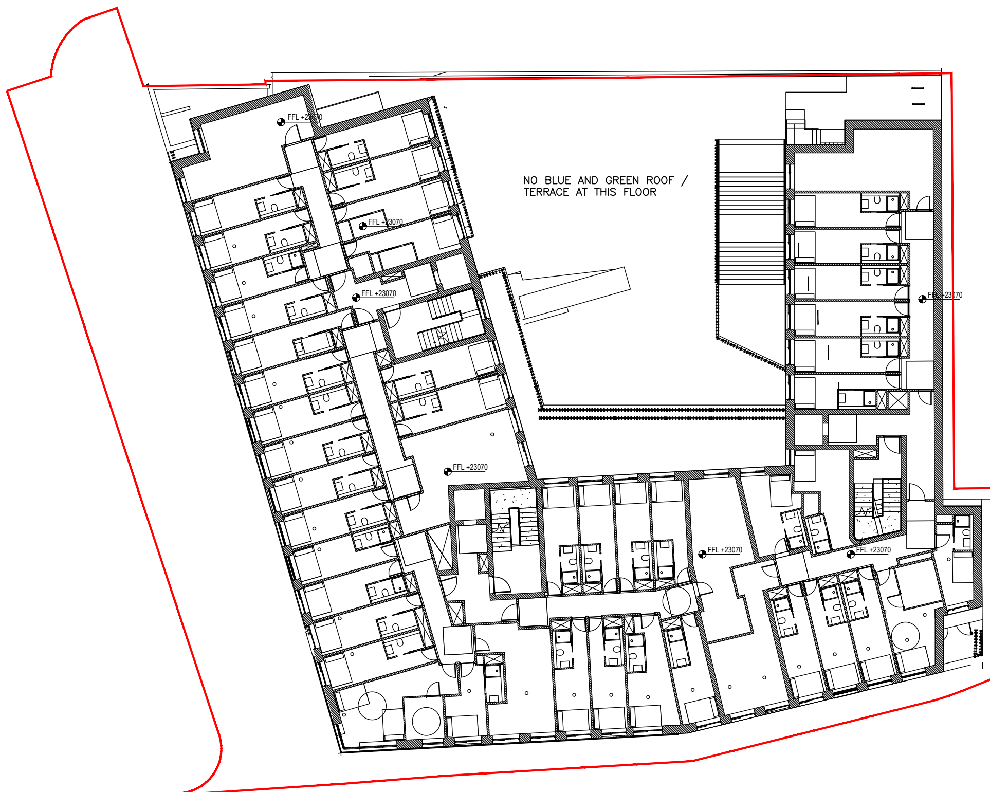
3 THIRD FLOOR PLAN SCALE 1:250
